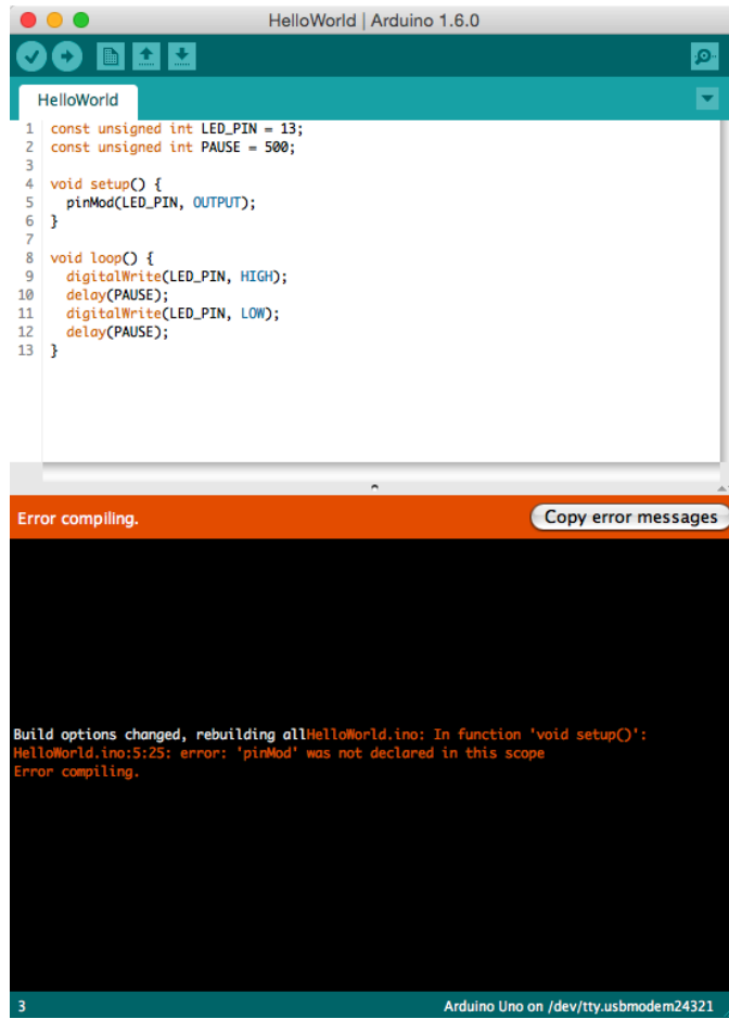
Figure 6—The Arduino IDE explains syntax errors nicely.
